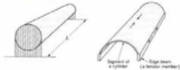
Cylinder → Tongewelf
