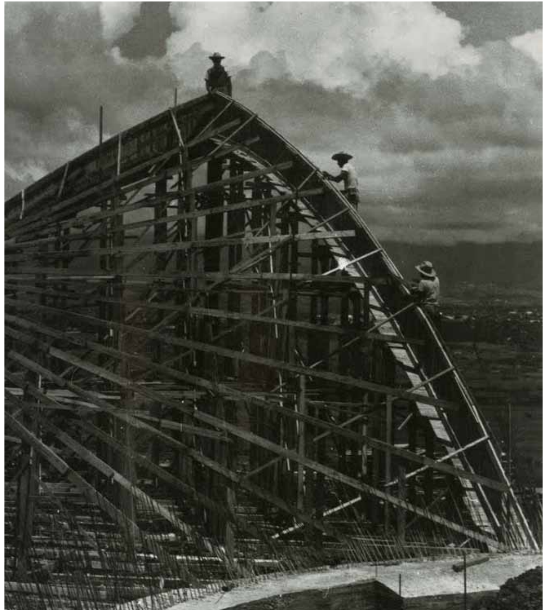
Open Chapel in Cuernavaca (1958) - Felix Candela
